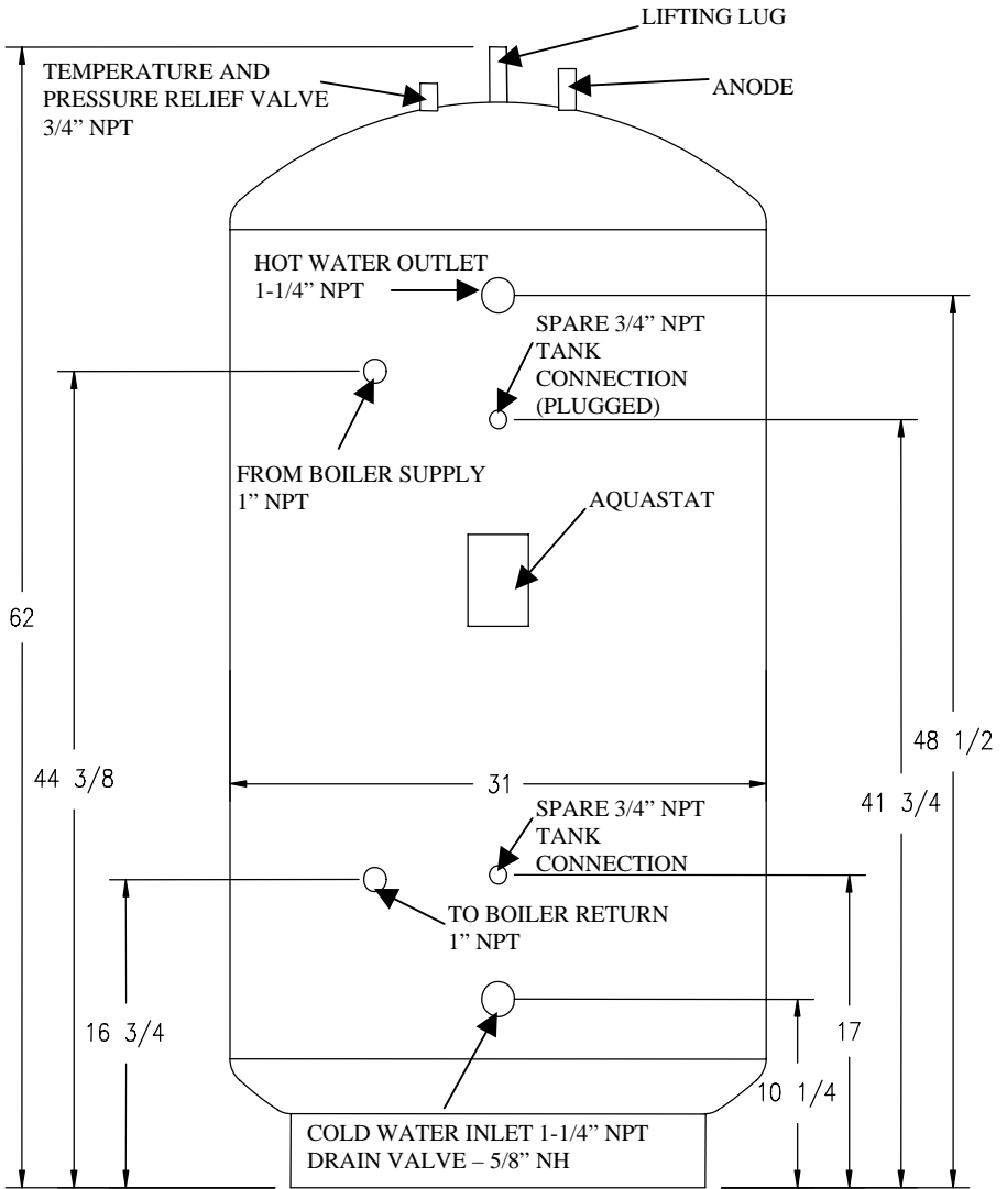
Figure 3 – Tank Layout (119 gallon model)
