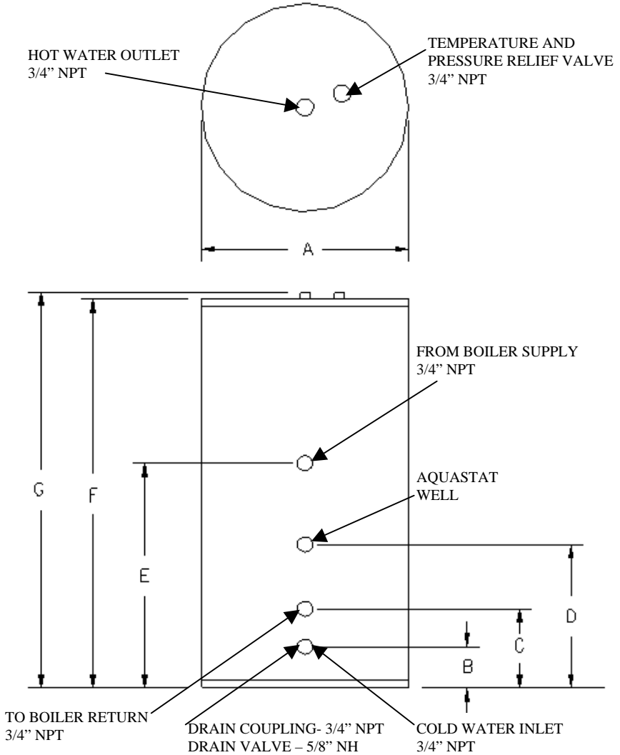
Figure 1 – Heater Layout (40, 52, 75 single exchanger models)
