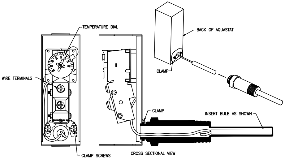
Figure 7 - Aquastat Control
