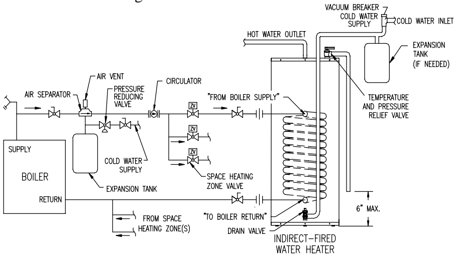
Figure 4 - Water Boiler Piping with Zone Valves
