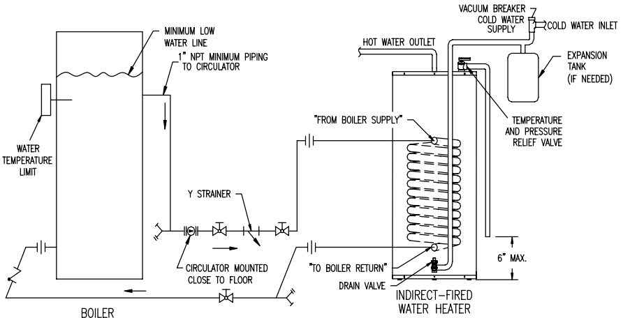
Figure 6 – Typical Steam Boiler Connections (connections available below the water line)
