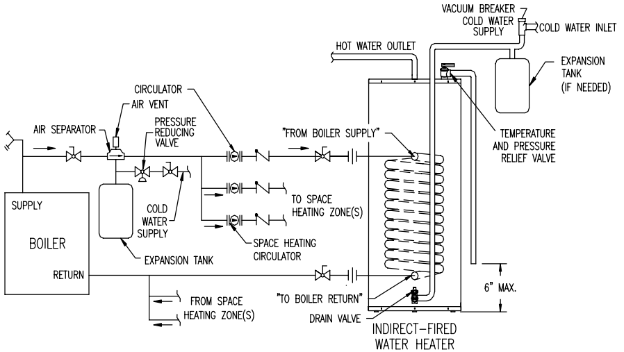
Figure 5 - Water Boiler Piping with Circulators
