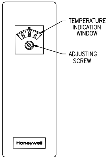
Figure 9 - Aquastat Control
