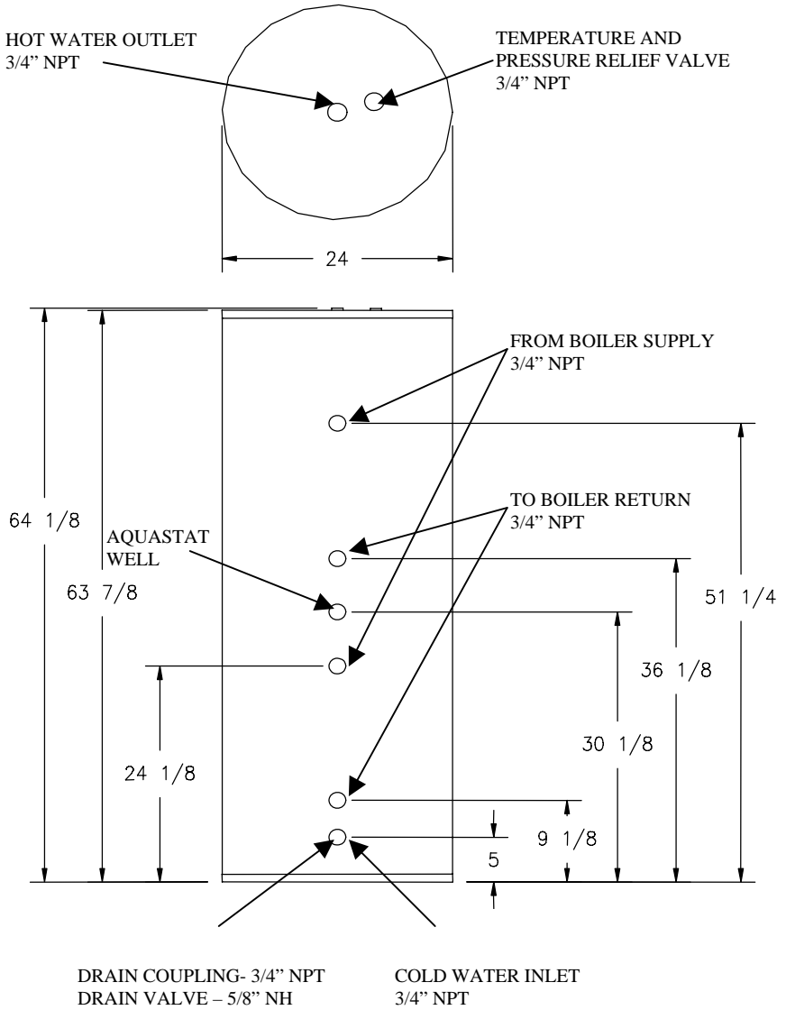
Figure 2 – Tank Layout (75 dual exchanger model)
